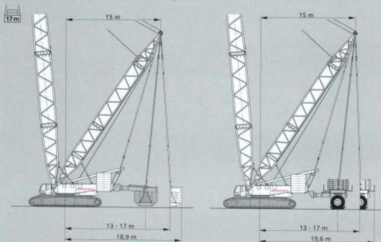
Variabel Superlift attachment - variable Superlifteinrichtung - Superlift variable
