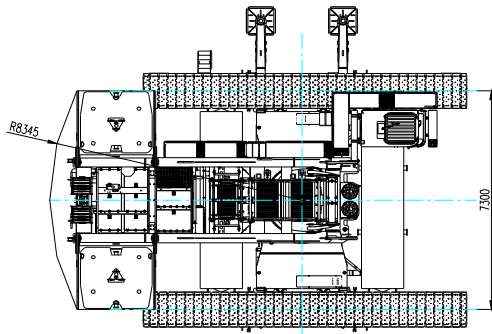
Fig. 1 XGC400-I crawler crane outline dimension (standard working condition)
