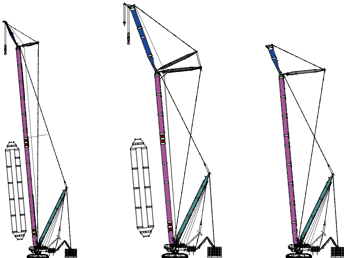
FJDB_7 (Boom 126~150m, jib 18m) Light fixed jib with superlift
