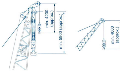
Main boom + auxiliary jib
